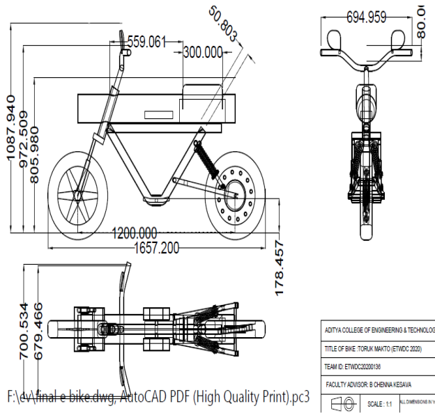
Master layout of Electric bike
